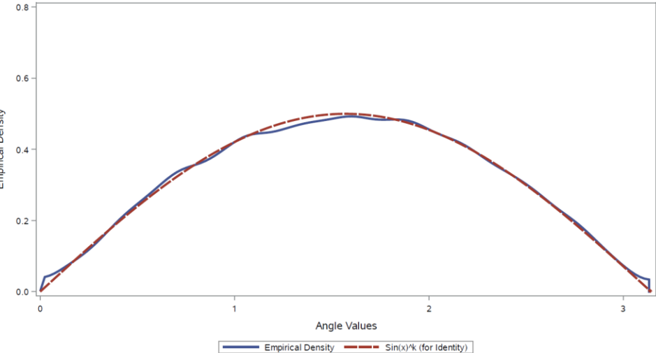
Angles v Identity (k=2)[row=4, Angle#=2]: DGM=C3, Mat=5x5, #Obs=6, #Sims = 10000
